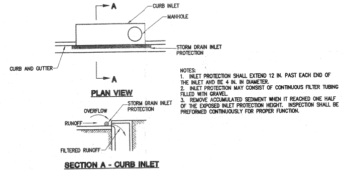
2 INLET PROTECTION - CDOT M-208-1 Scale: NOT TO SCALE
