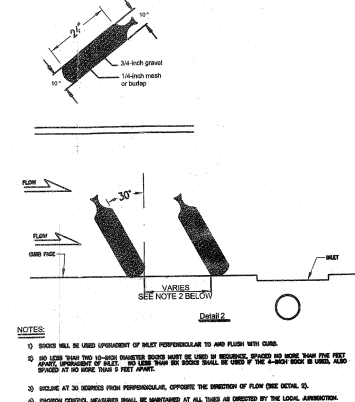
4 CURB SOCK INLET PROTECTION Scale: NOT TO SCALE
