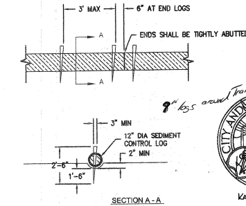
4 CURB SOCK INLET PROTECTION Scale: NOT TO SCALE
