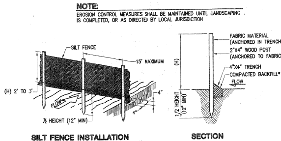
3 SILT FENCE EROSION BARRIER DETAIL Scale: NOT TO SCALE
