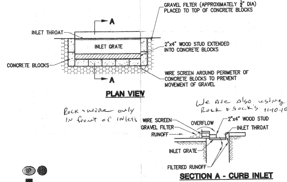
1 INLET PROTECTION - TYPE 18 Scale: NOT TO SCALE
