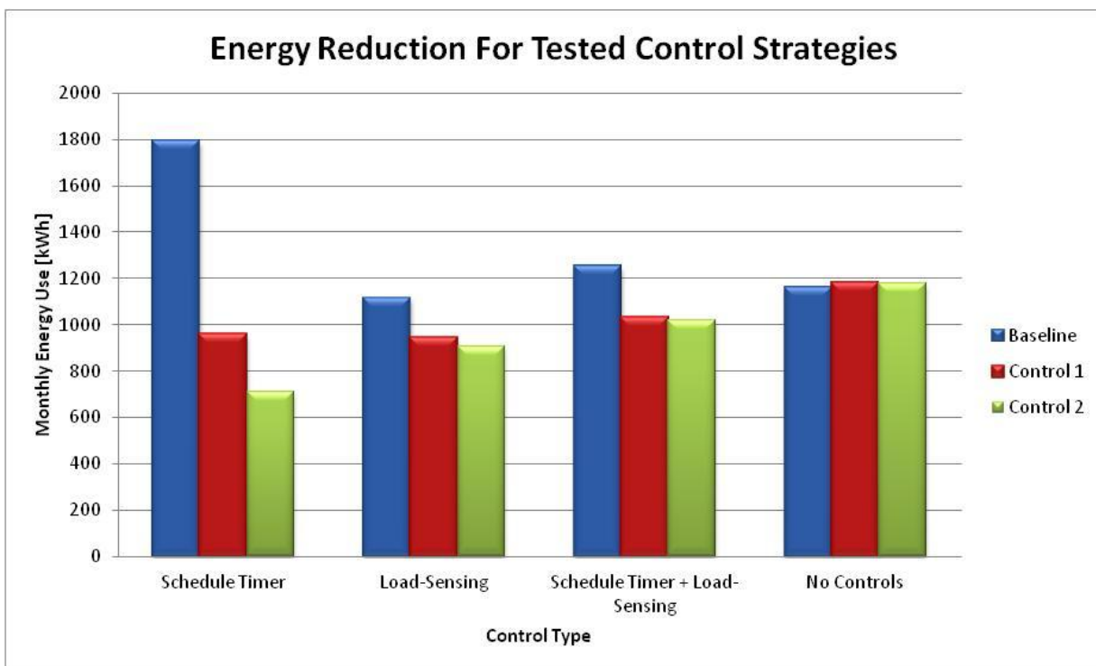
Figure V-1: Monthly energy reduction for tested control strategies
