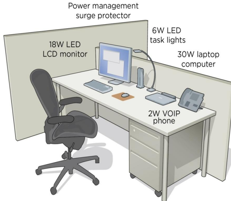
Figure VI-2: Example of low-energy workstation recommended as best practice. Credit: Mathew Luckwitz, NREL
