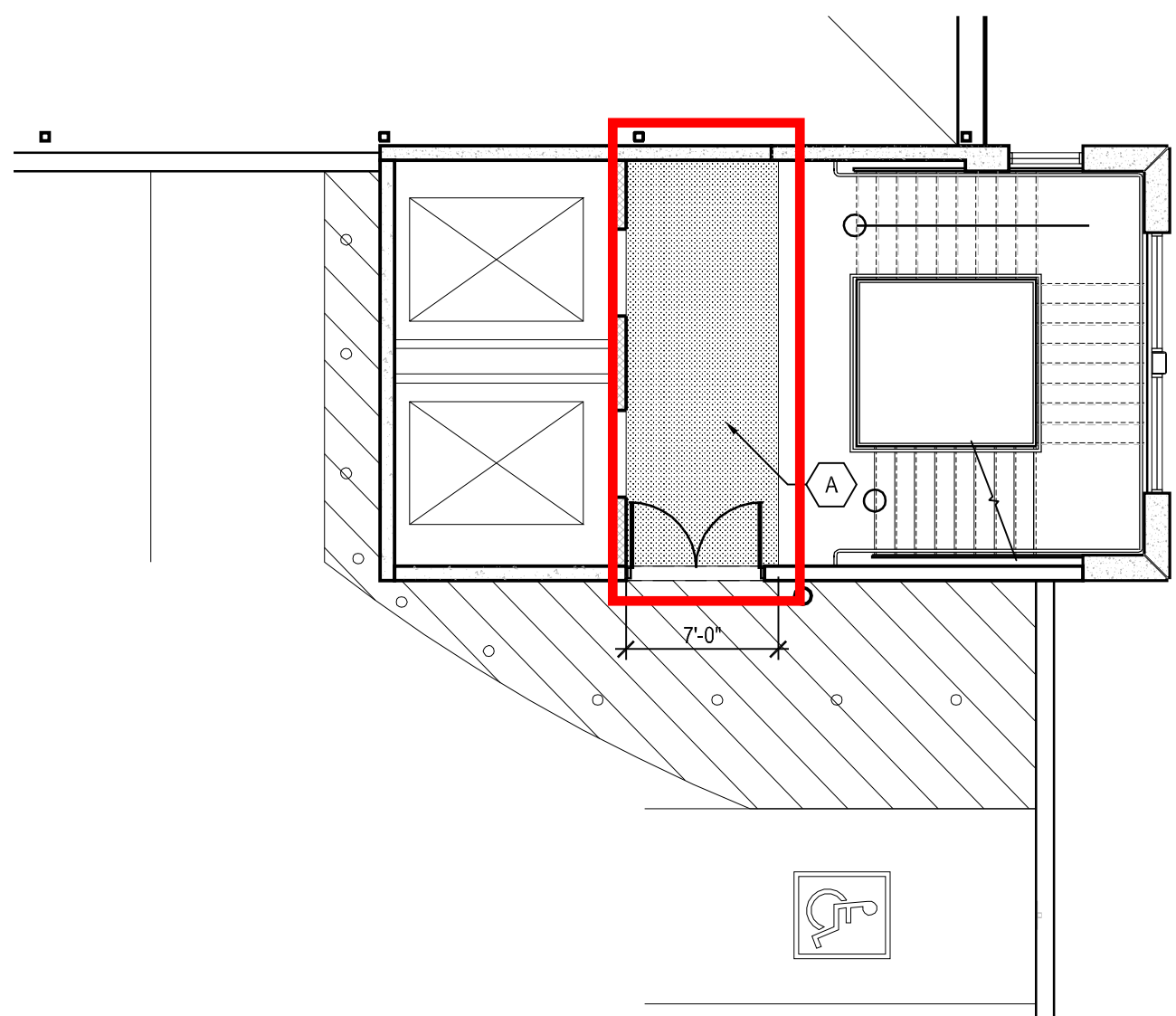
3 PARKING GARAGE LEVEL 2 ELEVATOR LOBBY 1/8" = 1'-0" NOTE: LEVELS 3-5 SAME/SIMILAR
